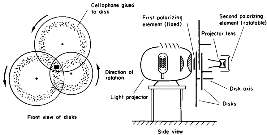
Fig. 1. Diagram of the 'Chromatic Abstractoscope'.
